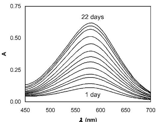
Figure 1. Spectrograms showing the formation of the sorbate–NBP adduct with time in 7:3 water/dioxane medium and variation in absorbance over the 1–22 day interval. [\text{S}]_0 = 0.2 M; [\text{HCl}] = 0.1 M; [\text{NBP}]_0 = 0.003 M; pH 5.5; T = 35 °C.
